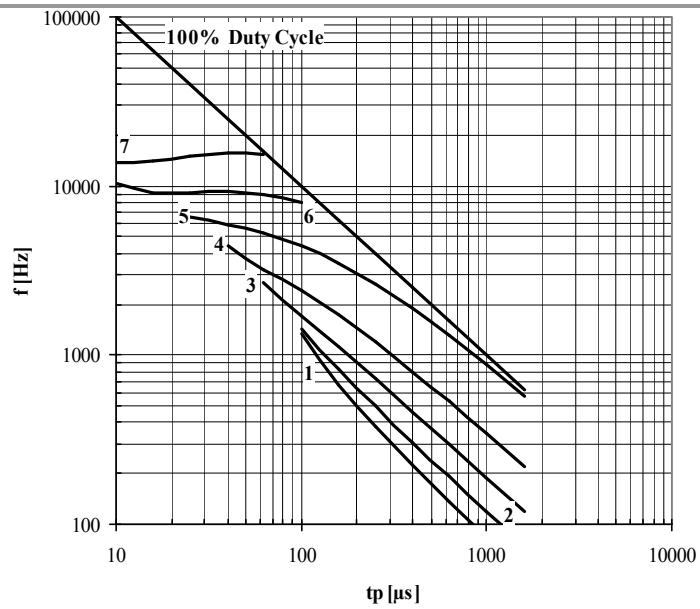
Fig. 18 Square wave frequency ratings
