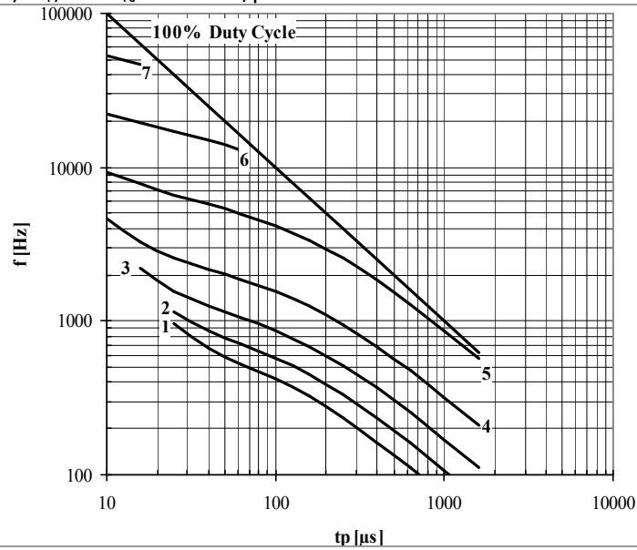
Fig. 15 Square wave frequency ratings
