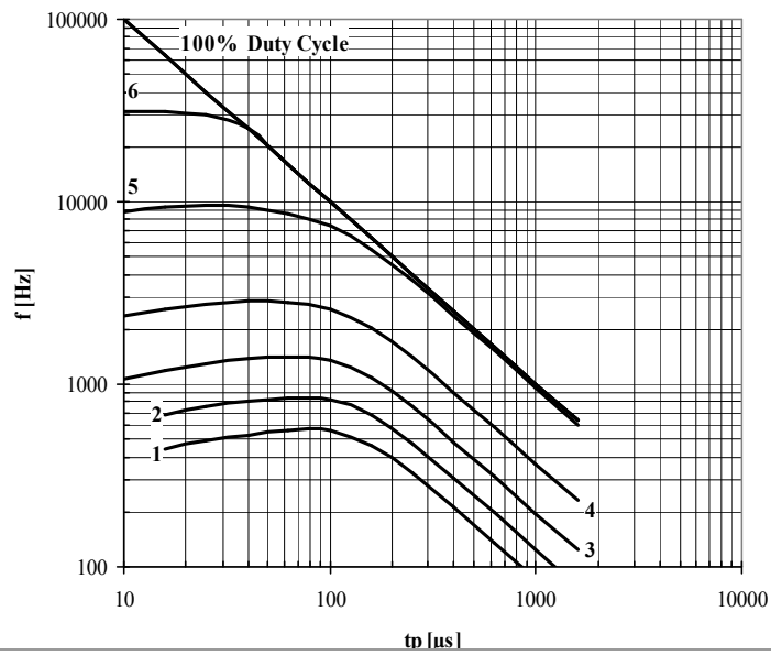
Fig. 11 Sine wave frequency ratings
