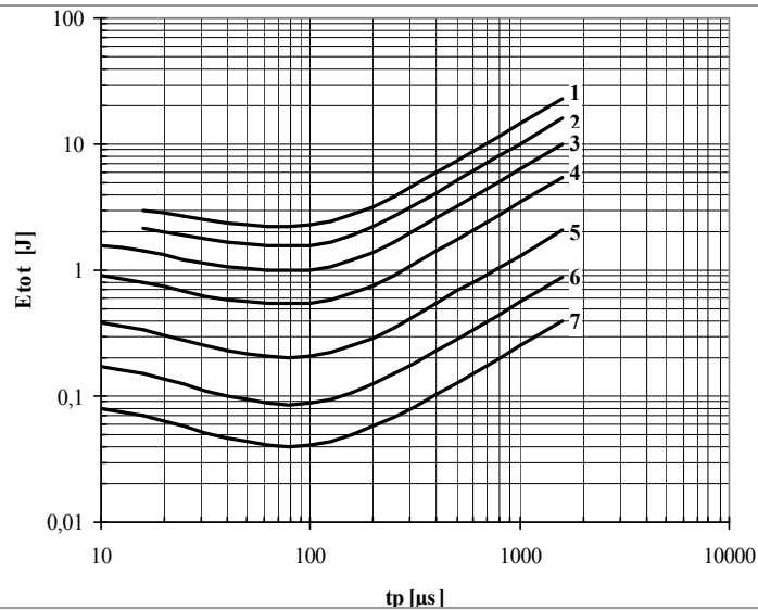
Fig. 23 Sine wave loss energy per pulse
