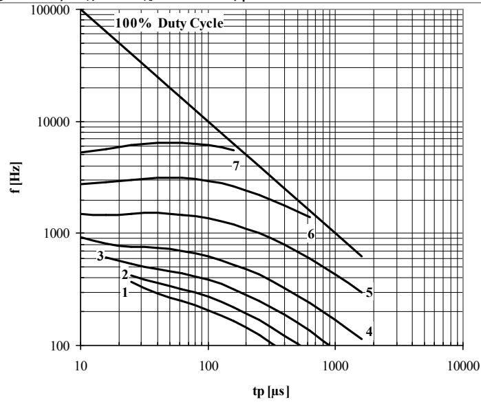
Fig. 21 Square wave frequency ratings
