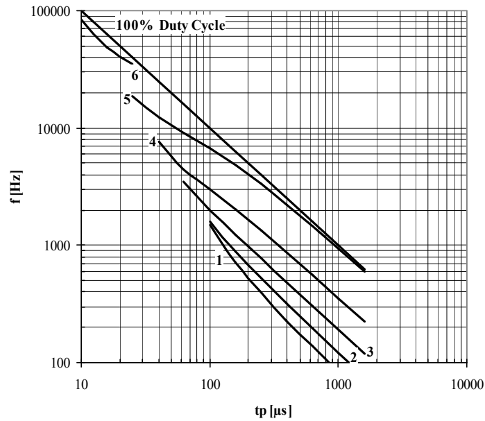
Fig. 14 Square wave frequency ratings
