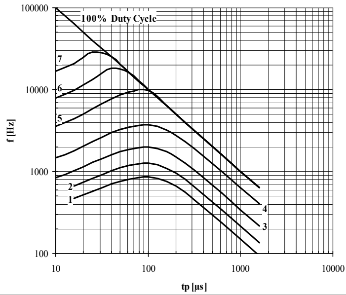
Fig. 12 Sine wave frequency ratings
