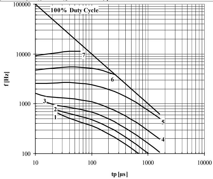
Fig. 19 Square wave frequency ratings
