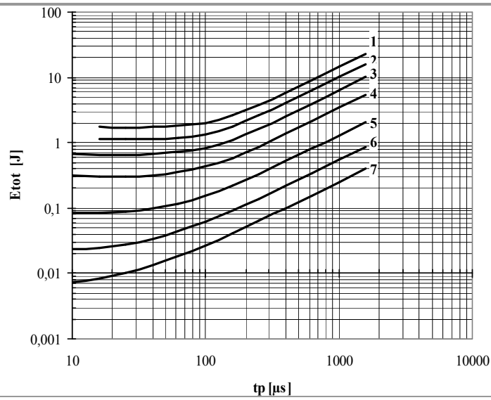
Fig. 22 Sine wave loss energy per pulse
