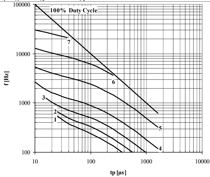
Fig. 17 Square wave frequency ratings
