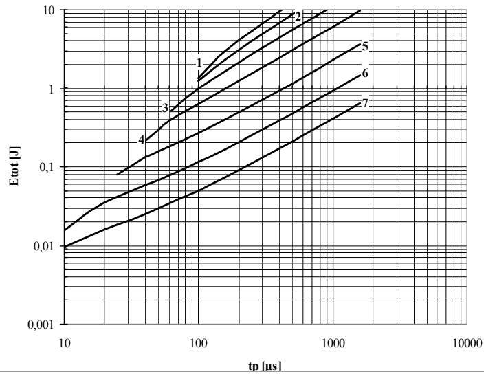
Fig. 24 Square wave loss energy per pulse
