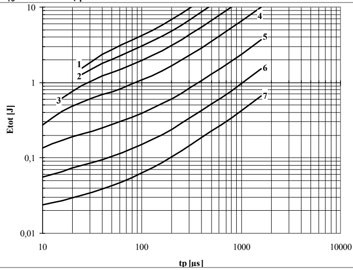
Fig. 25 Square wave loss energy per pulse
