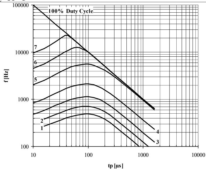
Fig. 13 Sine wave frequency ratings
