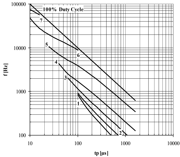
Fig. 16 Square wave frequency ratings
