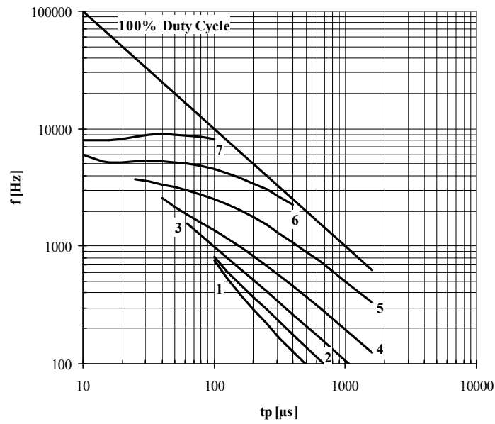
Fig. 20 Square wave frequency ratings
