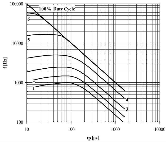
Fig. 10 Sine wave frequency ratings
